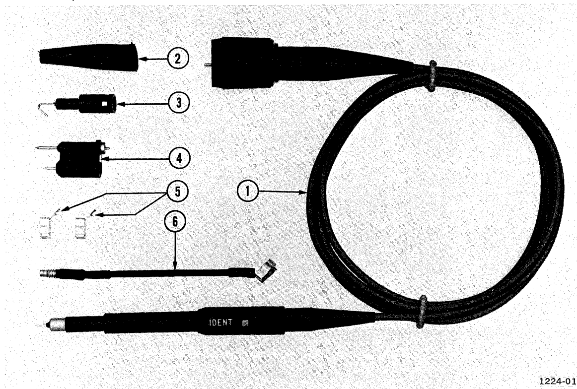
Fig. 1. P6056/P6057 probe with standard accessories.
