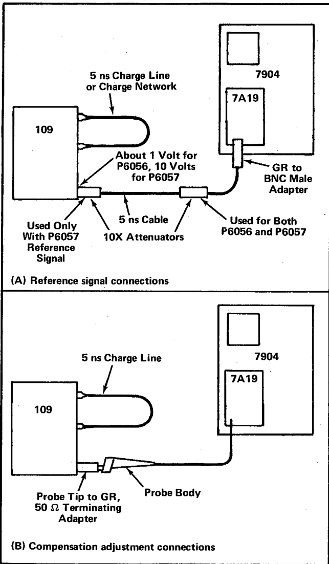
Fig. 2. Equipment setup for compensating the P6056 and P6057
